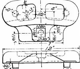
Figs. 4703-1. SIDE-BEARING (2).
